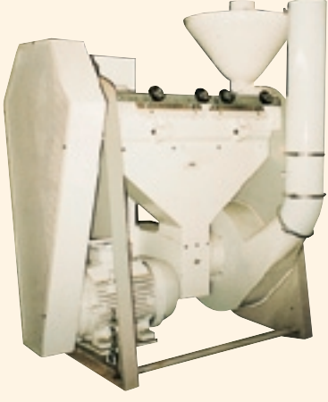
5 Polisher
